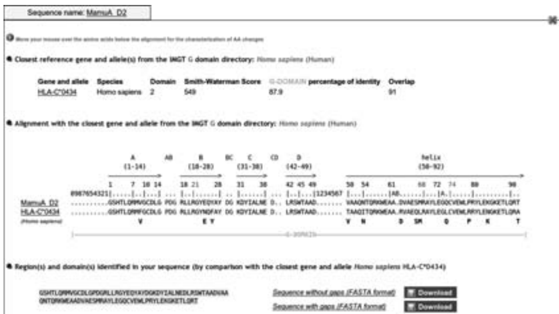
FIGURE 12. IMGT/DomainGapAlign top of the results page for a G domain, G-ALPHA2. G-ALPHA2 is the second domain of an MH1 chain. In this example, the user sequence is the G-ALPHA2 of MamuA (Macmul MH1-A) of the rhesus monkey Macaca mulatta aligned with the G-ALPHA2 of the closest human HLA-C allele.
