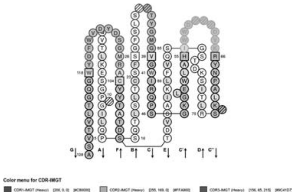
FIGURE 6. IMGT Collier de Perles of a V domain, on two layers, obtained after selection of “2” in Number of layers, “1 (RPI, IGH, TRB, TRD)” in CDR-IMGT color type, the domain belonging to an IGH chain, and by default “50% Hydrophobic positions.” Positions in blue mean that the amino acid of the user sequence at these positions is hydrophobic (hydropathy index with positive value) or is a tryptophan (W), like in 50% or more of analyzed V domains. Positions with red and bold letters indicate the five conserved positions of a V domain: 1st-CYS 23, CONSERVED-TRP 41, hydrophobic 89, 2nd-CYS 104, and J-TRP 118. Anchor positions are in squares. Hatched positions correspond to gaps according to the IMGT unique numbering for V domain (Lefranc 1997, 1999; Lefranc et al. 2003). Prolines are shown in yellow. Arrows indicate the \beta strands and their direction. The CDR-IMGT lengths of this domain are [10.7.13].
